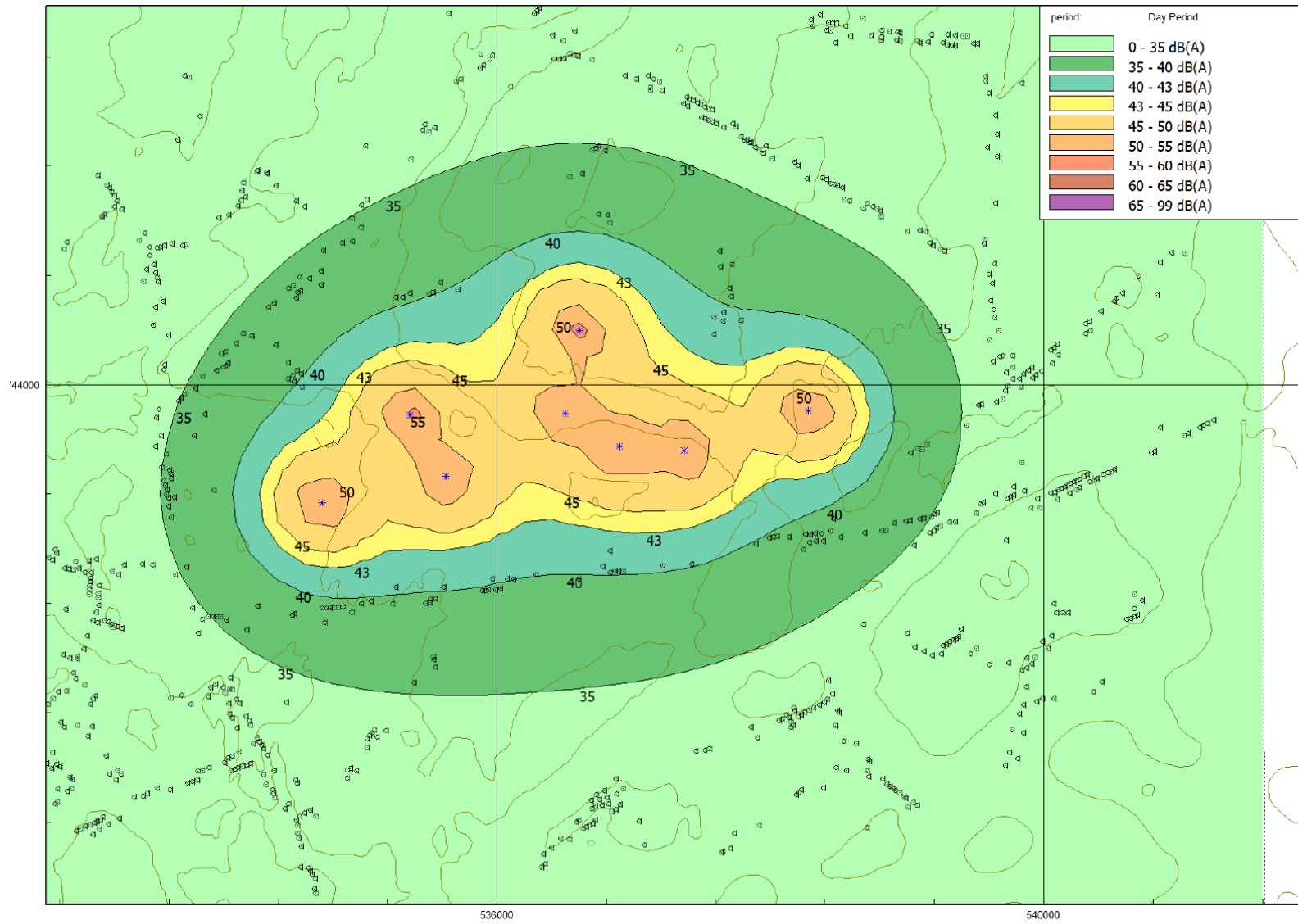
Figure 1 Predicted Noise Contours for wind speed of 8 m/s standardized for a hub height of 103.5 m
